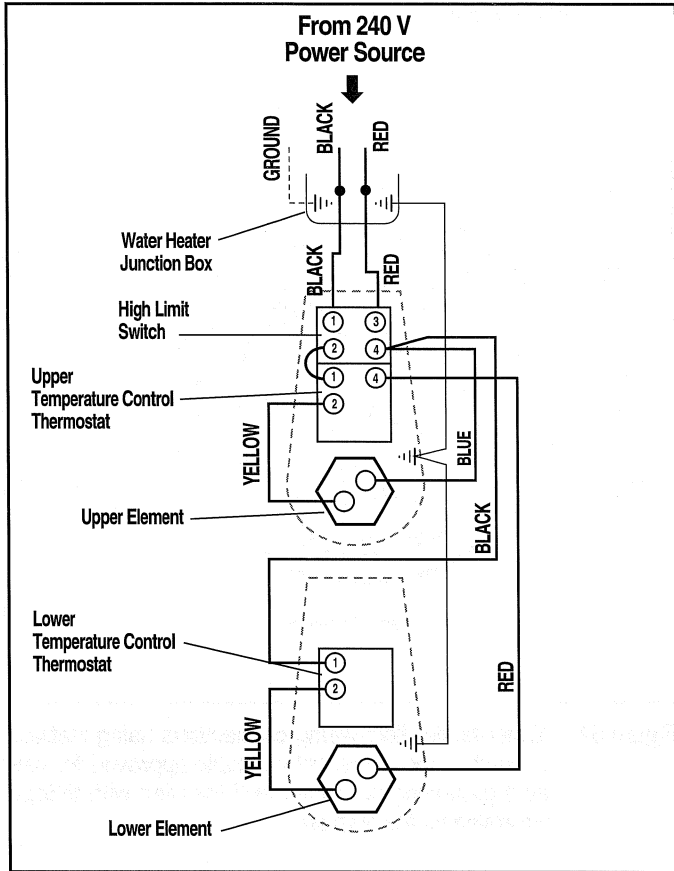
Figure 6 — Complete Wiring Schematic Diagram — Standard Non-Simultaneous Operation.
